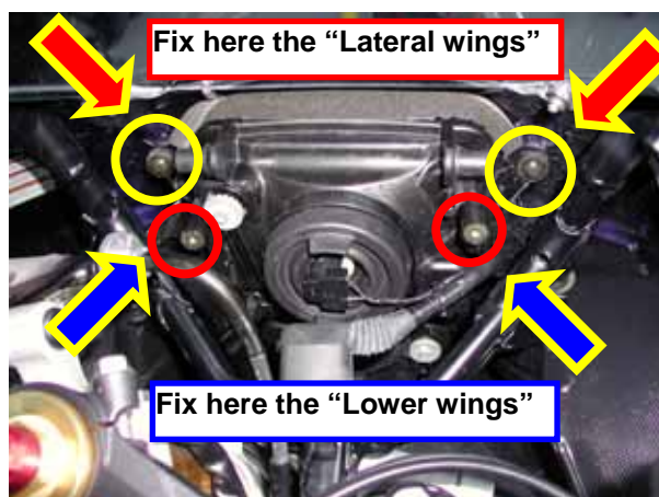
Figure 28: Lateral and lower “wings” fixing positions
