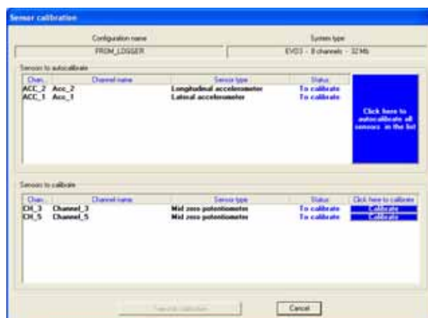
Figure 37: Race Studio 2 – Calibration window
